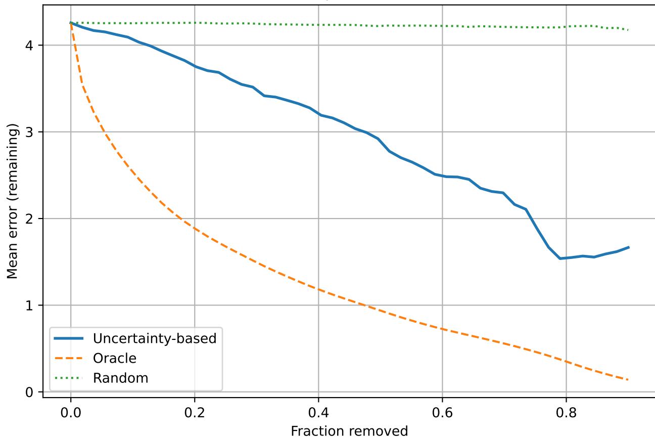
BPIC20DD: Sparsification Curve
